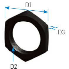
Lock Nut
