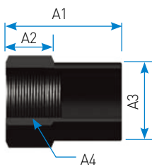
Stop Collar
